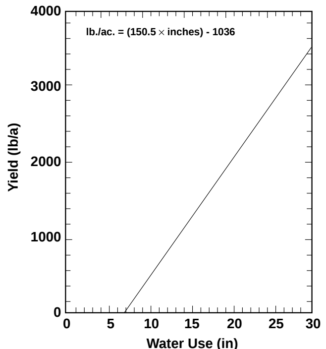
Figure 3. Sunflower yield as influenced by water use, Akron, CO
